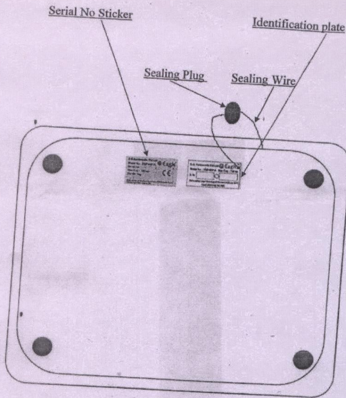
Figure- 2 Schematic diagram of the sealing arrangement
